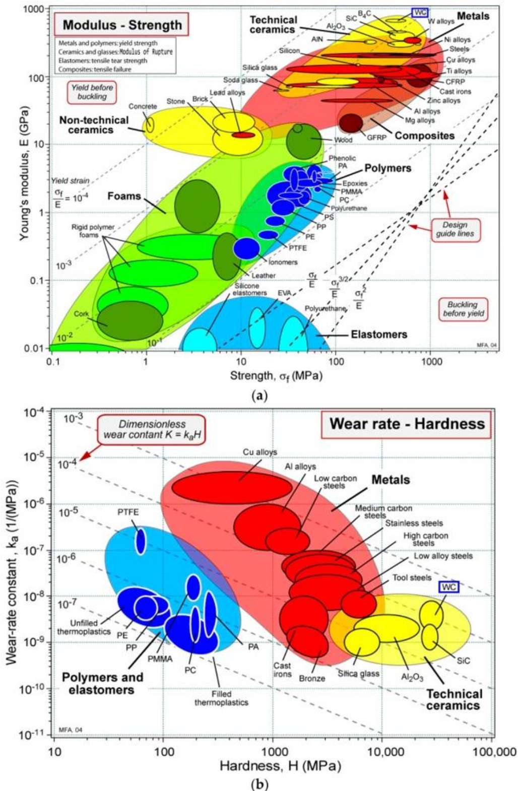
Figure 1. Ashby diagrams for different materials. (a) Young's modulus vs. strength, (b) wear-rate constant vs. Hardness (blue: polymers and elastomers, red: metals, yellow: technical ceramics) [1]
