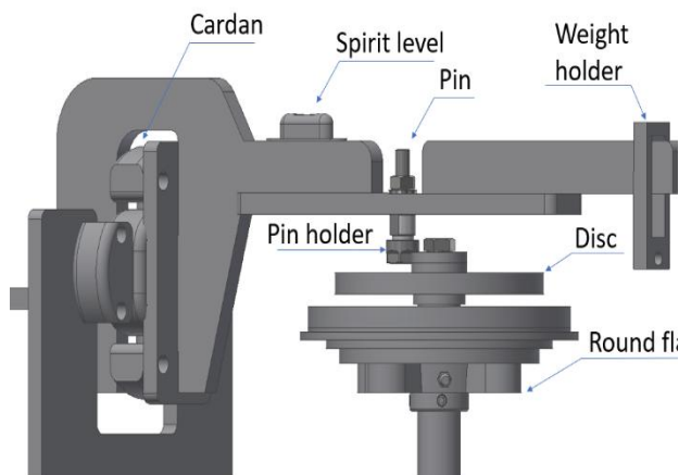
Figure 2. Main components of the tribometer
