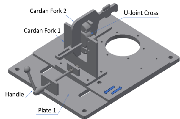
Figure 3 Construction of the Cardan joint with Plate 1 and the handle
