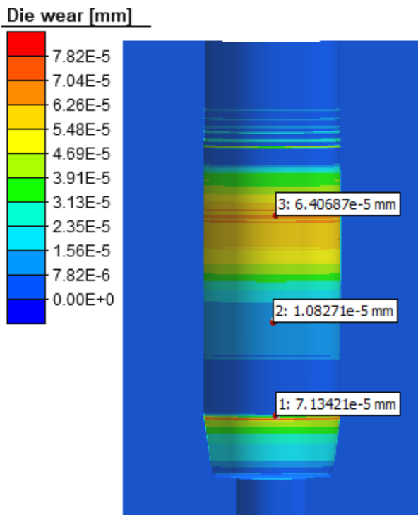
Figure 7. Die wear distribution in experiment 1
