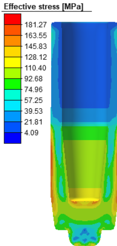
Figure 3. Distribution of effective stress on the workpiece (forging) in experiment 1
