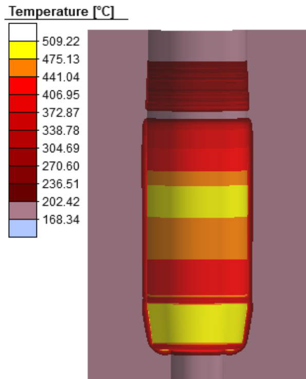
Figure 8. Temperature distribution on the die in experiment 1
