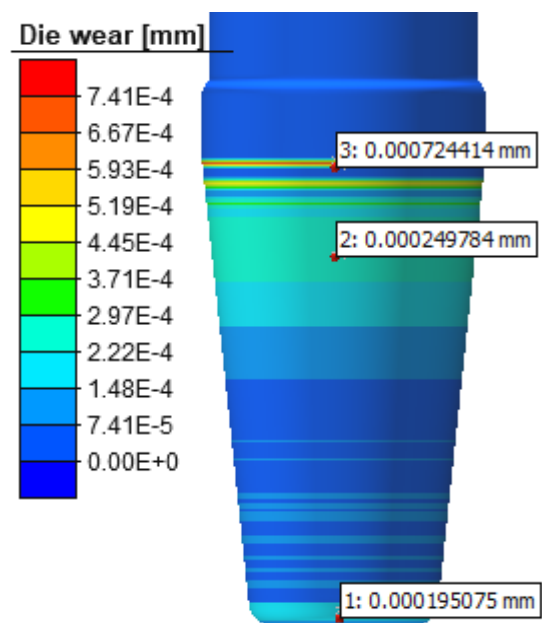
Figure 5. Wear distribution on the punch in experiment 1
