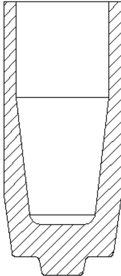
Figure 1. Forged shell body after hot forging
