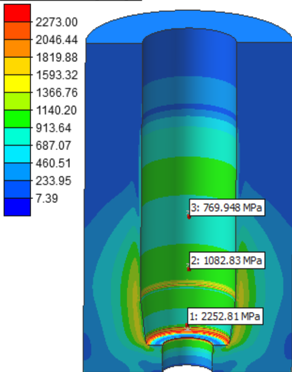
Figure 9. Distribution of effective stress on the die in experiment 1
