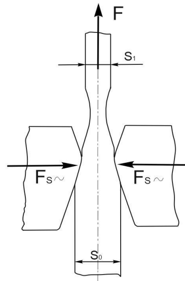
Figure 1. Scheme of the ironing process [5]
