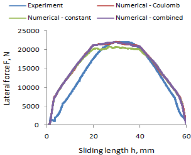
Figure 9. Lateral force diagram for DC04 material sheet strips
