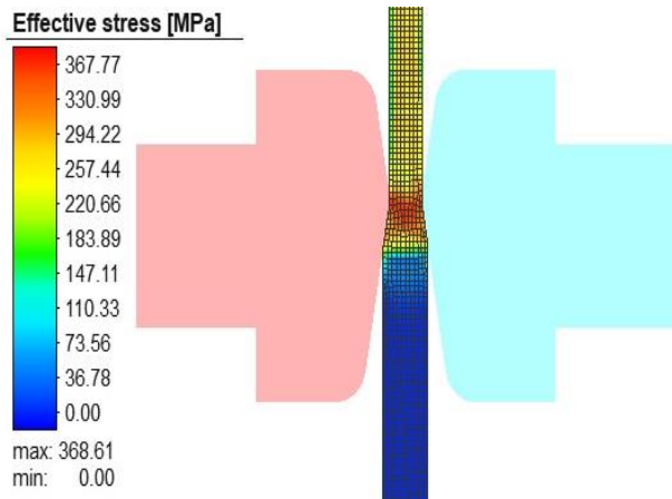
Figure 6. Effective stress distribution (DC04)
