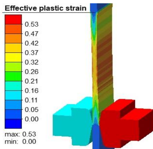
Figure 5. Effective plastic strain at the end of ironing process
