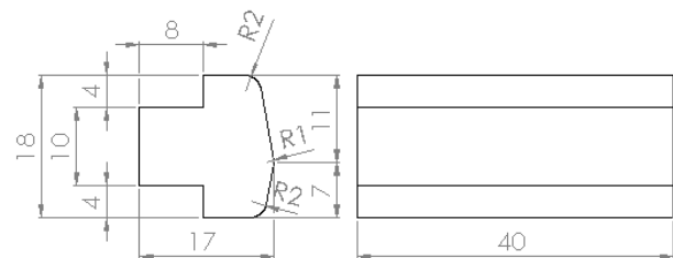
Figure 2. Drawing of the tool
