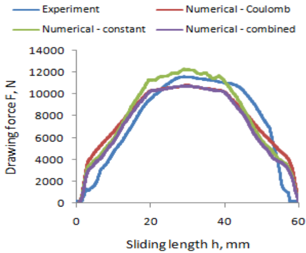
Figure 8. Drawing force diagram for DC04 material sheet strips
