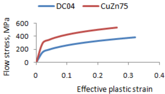
Figure 4. The flow curves
