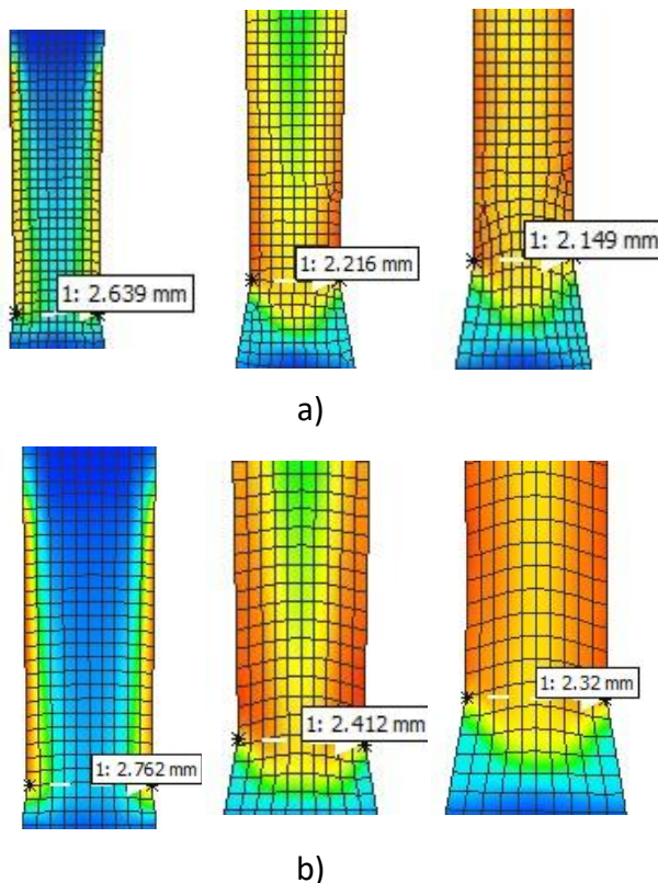
Figure 7. Sheet thickness after 10 mm, 20 mm and 30 mm of drawing length for a) DC04 b) CuZn75
