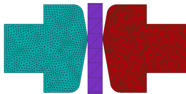
Figure 3. Tools and workpiece prepared for simulation
