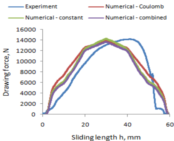
Figure 10. Drawing force diagram for CuZn75 material sheet strips
