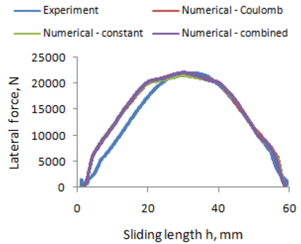
Figure 11. Lateral force diagram for CuZn75 material sheet strips
