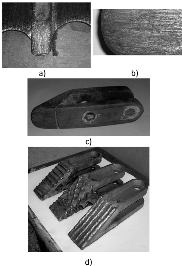
Figure 1. Display of teeth before and after hard-facing
