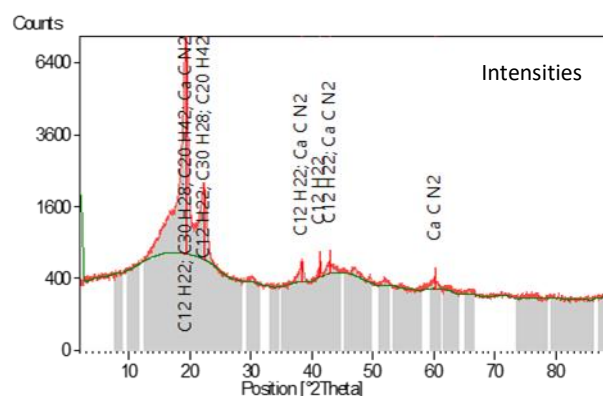
Figure 4. X-ray diffractograms of 4wt% eggshell particle reinforced low-density polyethylene
