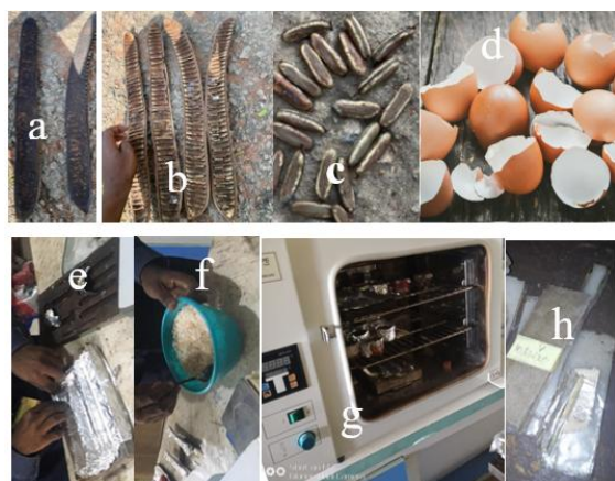
Figure 2. Pictorial demonstration of materials used and procedures for composite preparations: (a) Delonix regia fruits (b) Delonix regia pods (c) Delonix regia seeds (d) eggshells (e) mould lining with aluminium foil (f) oil-polyethylene-particles mixture ready to be poured into the mould (f) prepared low-density polyethylene based composites (g) Uniscope laboratory oven for heating the polymer (h) prepared composite samples
