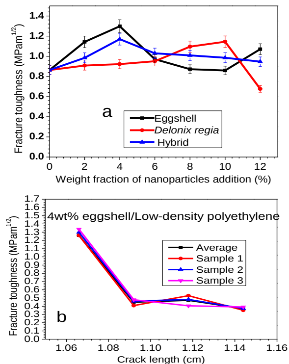
Figure 8. (a) Fracture toughness of the low-density polyethylene-based composites (b) Crack size with the fracture toughness of 4wt% eggshell particle reinforced low-density polyethylene
