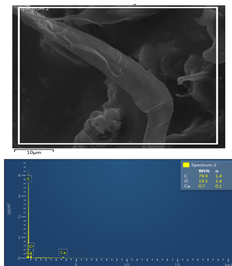
Figure 6. SEM/EDX of composite
