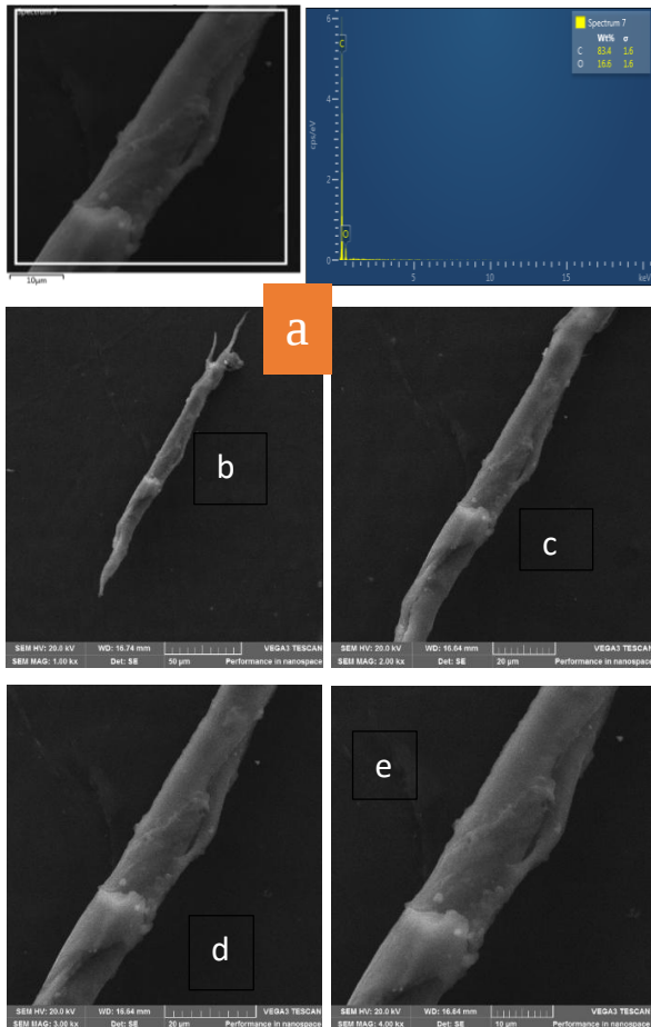
Figure 5. SEM/EDX of the pristine low-density polyethylene (a) chemical composition obtained from the area scanning of the polyethylene structure at resolution of 10 \mu\text{m} (b-d) images captured at different magnifications
