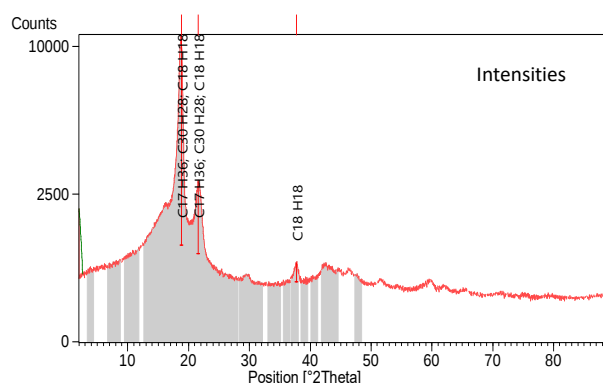
Figure 3. X-Ray Diffractograms of the Low-Density Polyethylene
