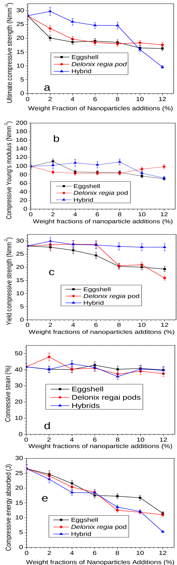
Figure 9. Compressive Properties of the Low-Density Polyethylene-Based Composites
